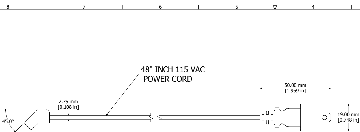
SIDE VIEW
