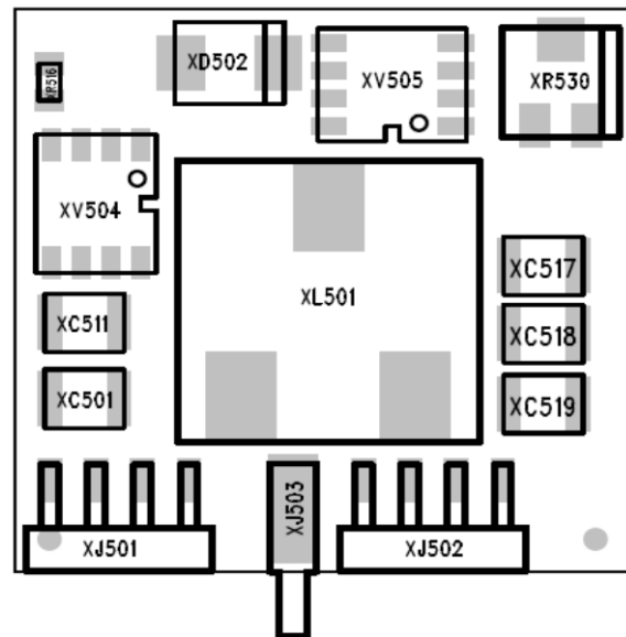
SMA 2 channel 3 board (SMA 3 channel 4 THV, FHV)
