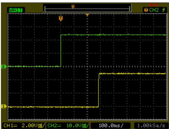
Figure 15: AXA02A18-L Output Voltage Startup Characteristic by ON/OFF Vin = 24Vdc Load: Io = 2A Ch1: Vo Ch2: Remote On/Off
