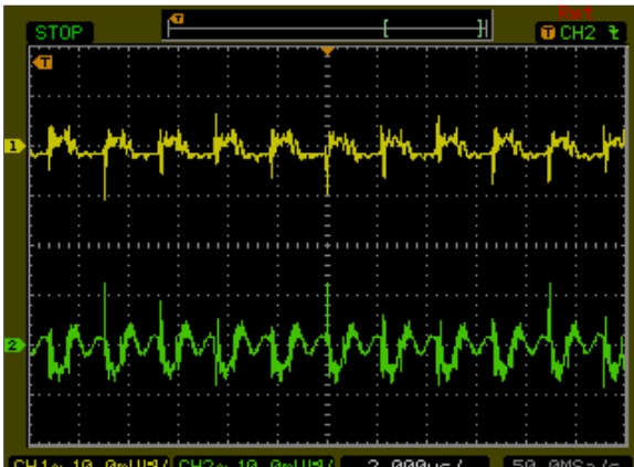
Figure 63: AXA000BB18-L Ripple and Noise Measurement Vin = 24Vdc Load: Io = ±0.41 A Ch 1: Vo1 Ch 2: Vo2
