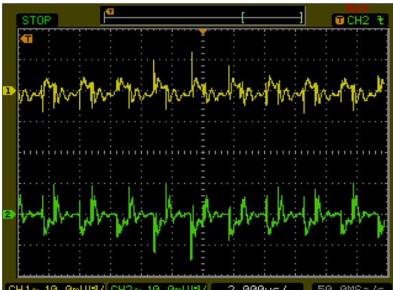
Figure 73: AXA000CC18-L Ripple and Noise Measurement Vin = 24Vdc Load: Io = ±0.33 A Ch 1: Vo1 Ch2: Vo2
