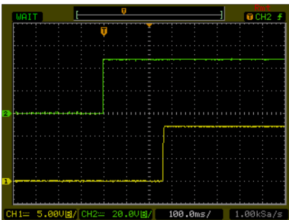
Figure 145: AXA000BB36-L Output Voltage Startup Characteristic by ON/OFF Vin = 48Vdc Load: Io = ±0.41 A Ch1: Vo Ch2: Remote On/Off
