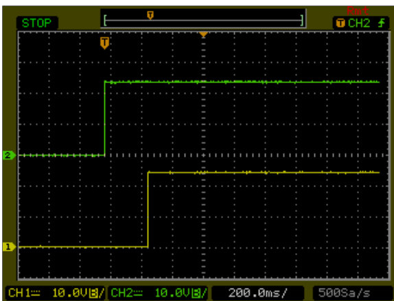
Figure 45: AXA000H18-L Output Voltage Startup Characteristic by ON/OFF Vin = 24Vdc Load: Io = 0.41A Ch1: Vo Ch2: Remote On/Off
