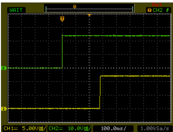
Figure 25: AXA00B18-L Output Voltage Startup Characteristic by ON/OFF Vin = 24Vdc Load: Io = 0.83A Ch1: Vo Ch2: Remote On/Off
