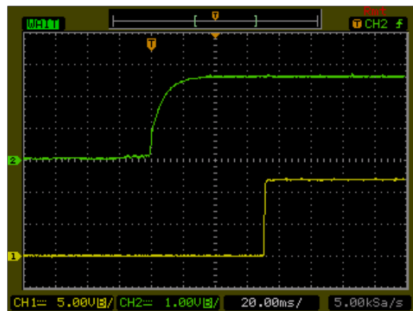
Figure 26: AXA00B18-L Output Voltage Startup Characteristic by Vin Vin = 24Vdc Load: Io = 0.83A Ch1: Vo Ch2: Vin
