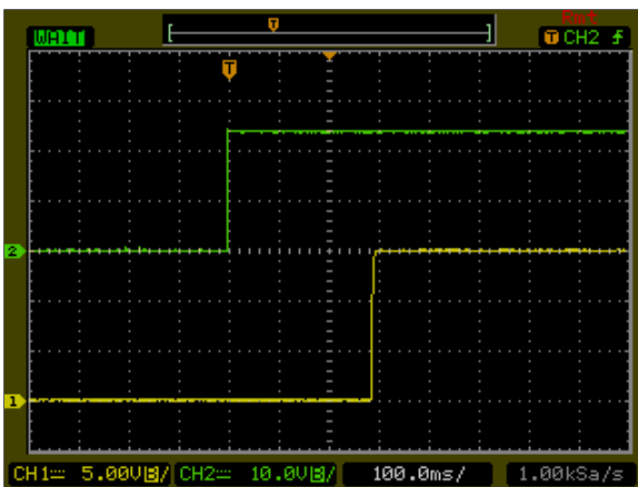
Figure 75: AXA000CC18-L Output Voltage Startup Characteristic by ON/OFF Vin = 24Vdc Load: Io = ±0.33 A Ch1: Vo Ch2: Remote On/Off
