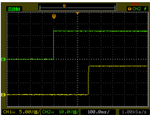
Figure 66: AXA000BB18-L Output Voltage Startup Characteristic by ON/OFF Vin = 24Vdc Load: Io = ±0.41 A Ch1: Vo Ch2: Remote On/Off
