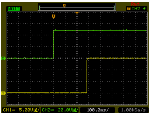
Figure 115: AXA00C36-L Output Voltage Startup Characteristic by ON/OFF Vin = 48Vdc Load: Io = 0.67A Ch1: Vo Ch2: Remote On/Off
