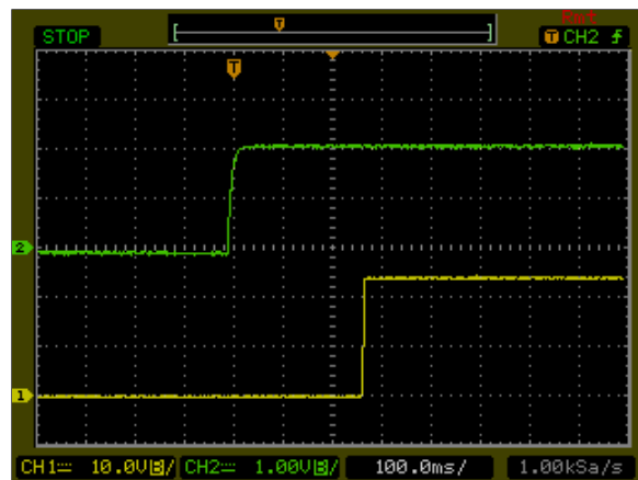
Figure 46: AXA000H18-L Output Voltage Startup Characteristic by Vin Vin = 24Vdc Load: Io = 0.41A Ch1: Vo Ch2: Vin
