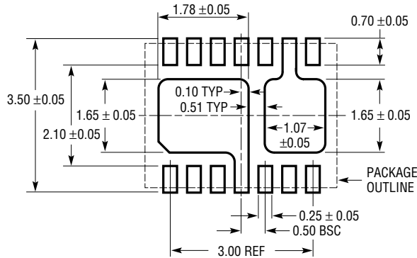
DE14MA Package 14-Lead Plastic DFN, Multichip (4mm × 3mm) (Reference LTC DWG # 05-08-1731 Rev 0)
