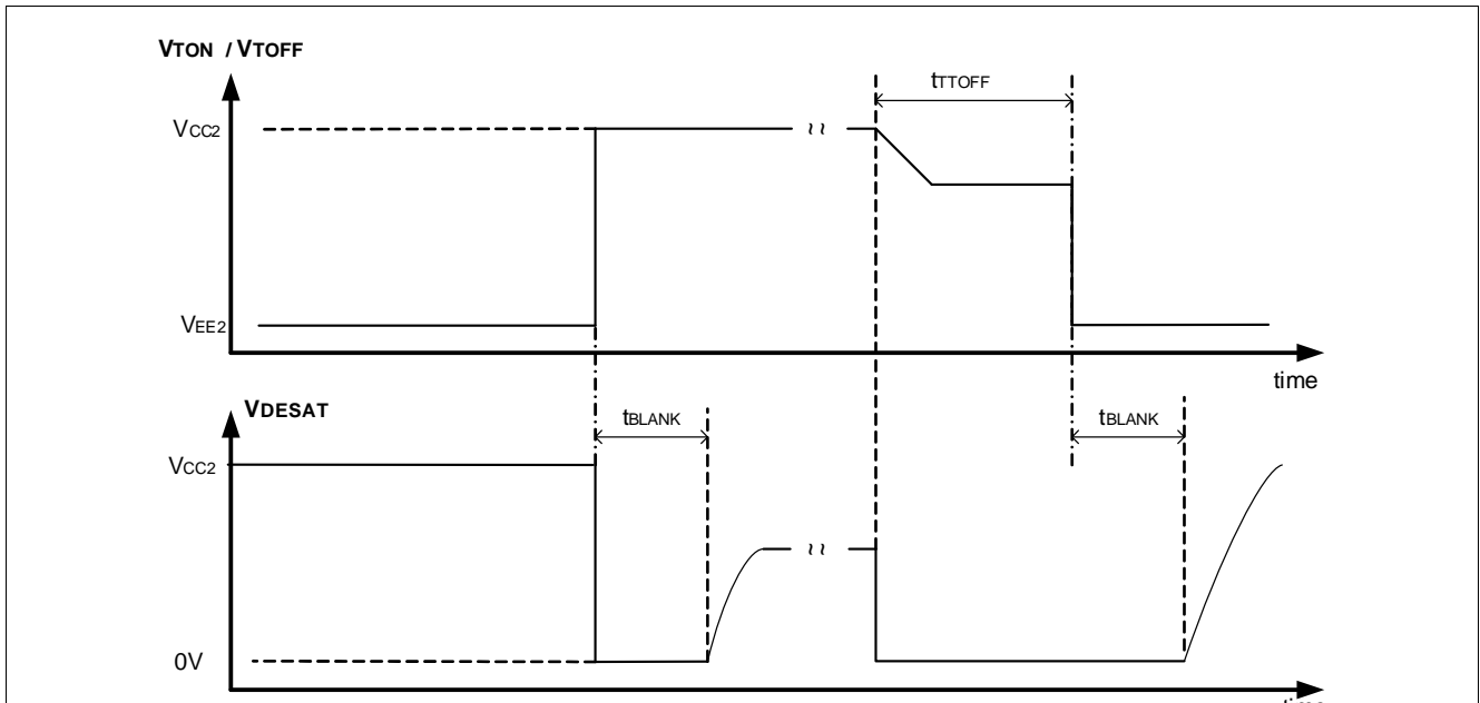
Figure 3-2 DESAT Operation
