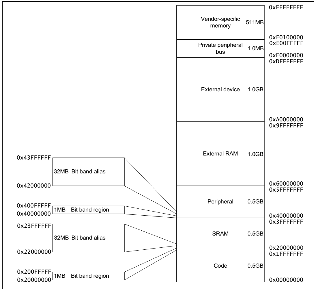
Figure 9. Memory map
