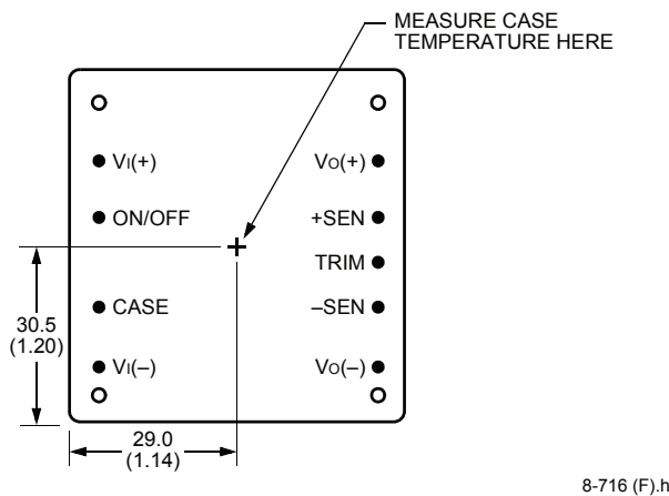
Figure 26. Case Temperature Measurement Location
