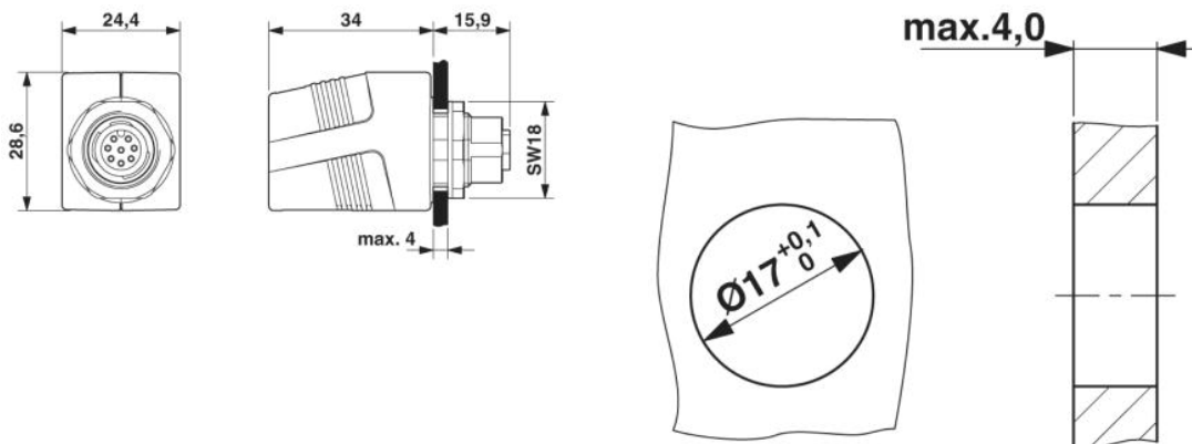
Panel cutout
