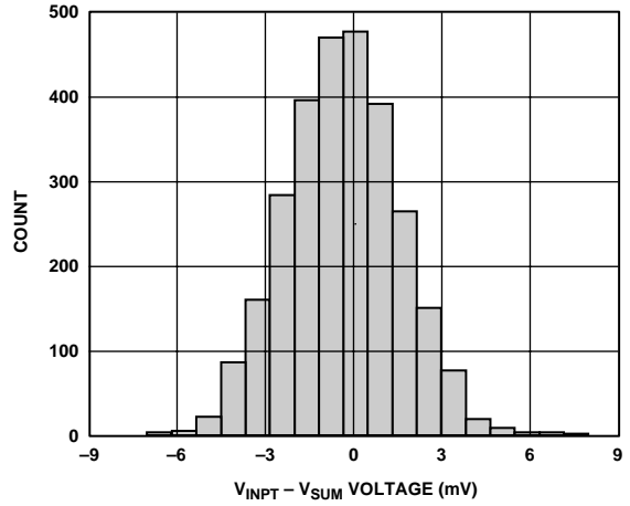
Figure 32. Distribution of Offset Voltage ( V_{INPT} - V_{SUM} )
