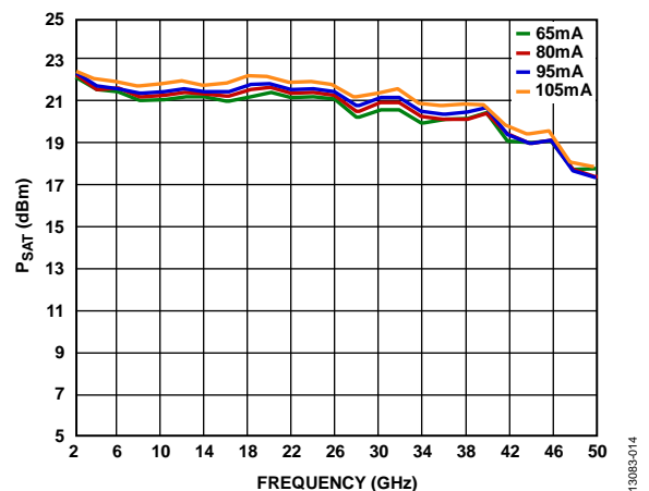
Figure 20. P_{SAT} vs. Frequency at Various Supply Currents (For V_{DD} = 5\text{ V} , V_{GG2} = 1.4\text{ V} )
