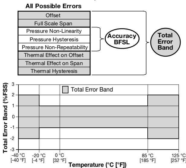
Figure 1. TEB Definition and Temperature Performance
